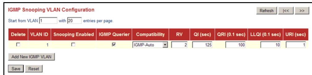
Figure 57: Configuring VLAN Settings for IGMP Snooping and Query
