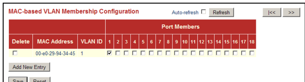
Figure 70: Configuring MAC-Based VLANs
