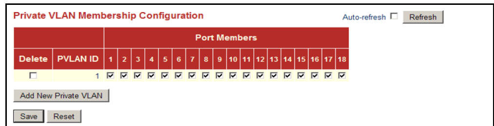
Figure 68: Private VLAN Membership Configuration
