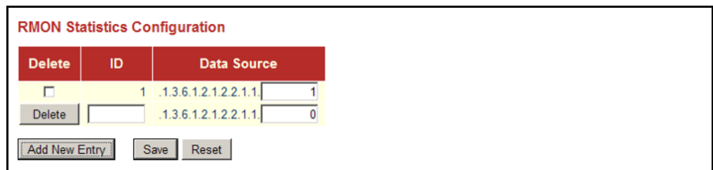
Figure 25: RMON Statistics Configuration
