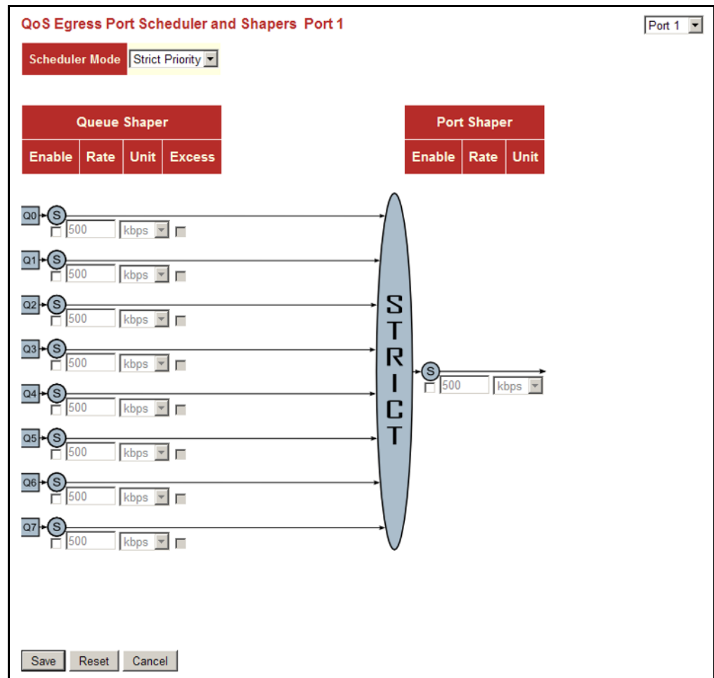
Figure 80: Configuring Egress Port Schedulers and Shapers
