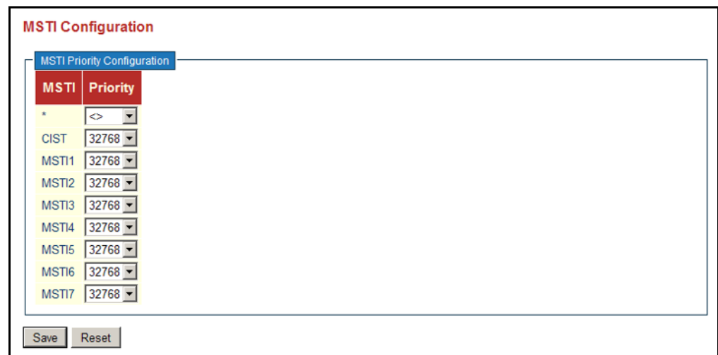
Figure 50: Configuring STA Bridge Priorities
