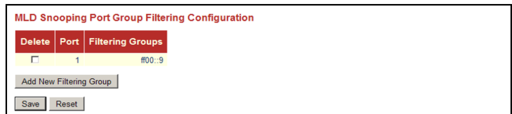
Figure 61: MLD Snooping Port Group Filtering Configuration
