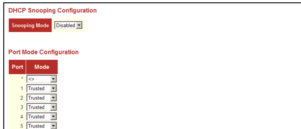
Figure 35: DHCP Snooping Configuration
