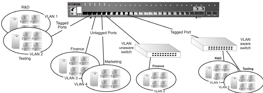
Figure 8: Making VLAN Connections
