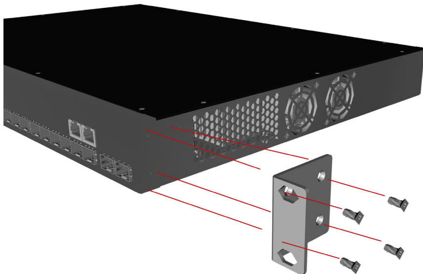
Figure 10: Attaching the Brackets
