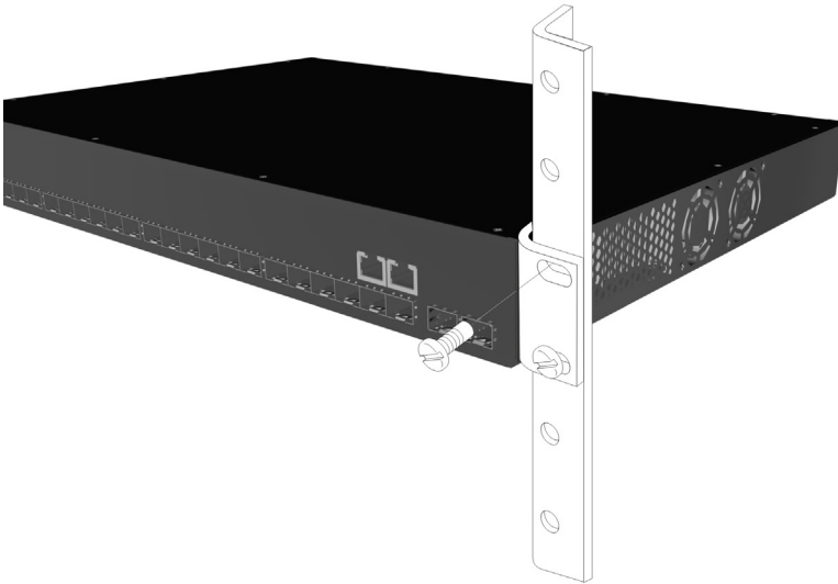
Figure 11: Installing the Switch in a Rack
