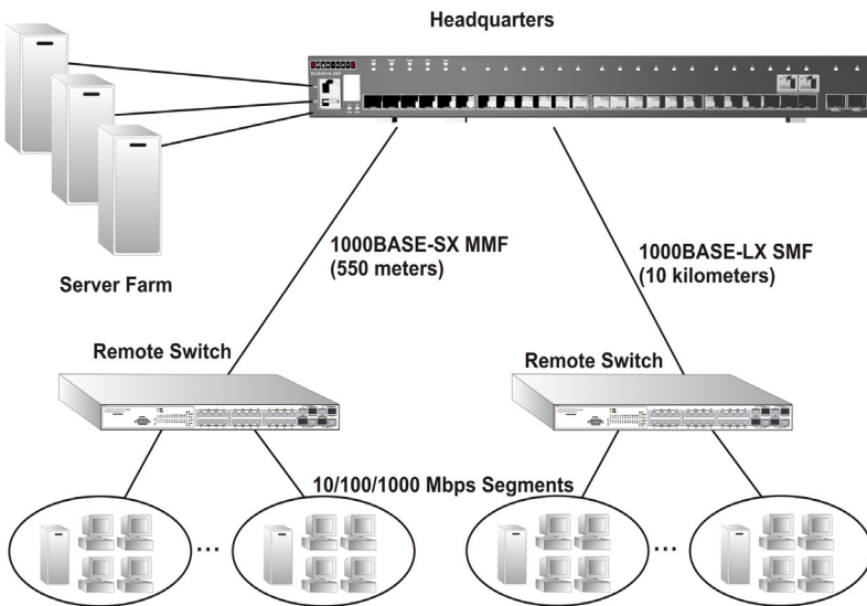
Figure 7: Remote Connections with Fiber Cable
