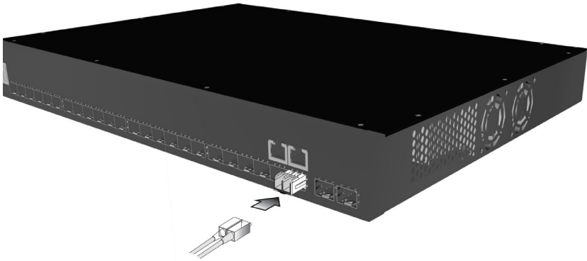
Figure 17: Making Fiber Port Connections
