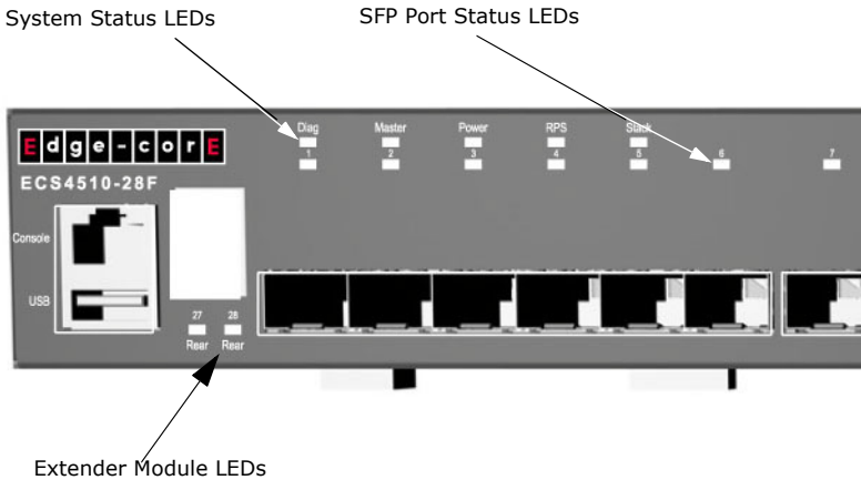
Figure 4: Port and System Status LEDs
